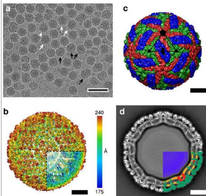
Figure 2: TBEV particles
